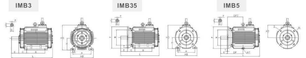
外形及安装尺（无风叶风罩） INSTALLATION AND OVERALL DIMENSIONS (WITHOUT FAN AND COVER)
