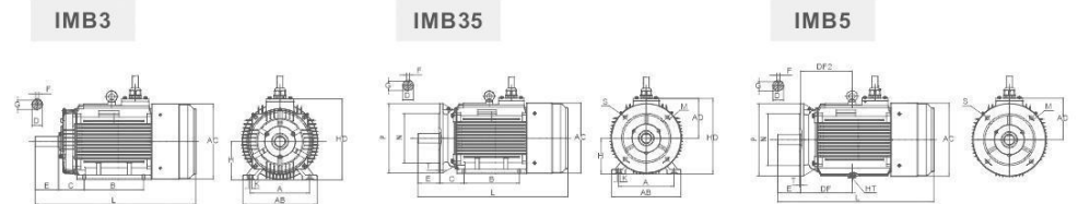
外形及安装尺（带风叶、风罩） INSTALLATION AND OVERALL DIMENSIONS (WITH FAN AND COVER)
